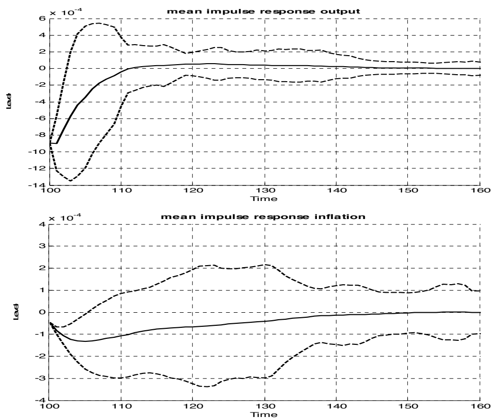
Figure 8: Mean impulse responses to an interest rate shock in the extended heuristic model
