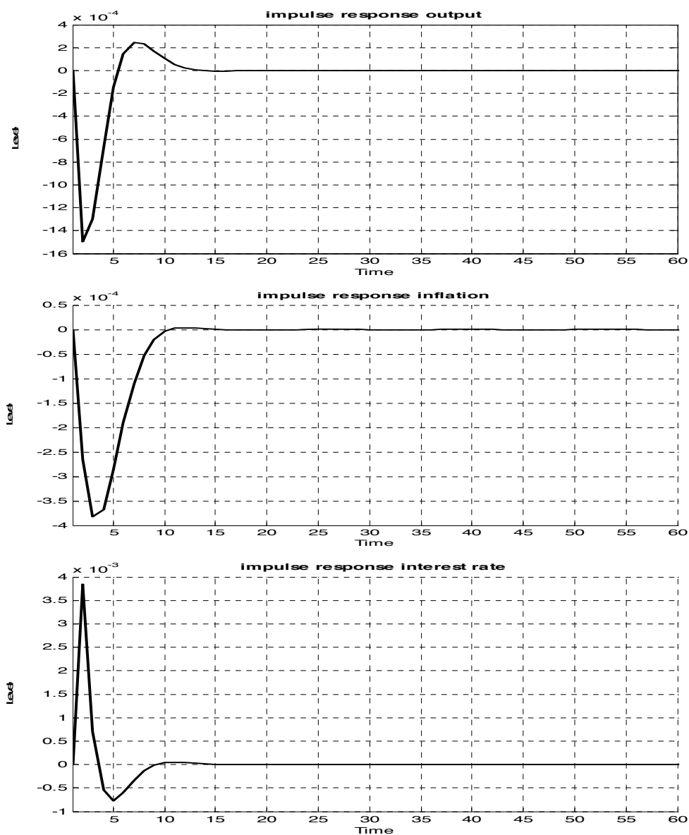
Figure 4: Impulse responses to interest rate shock in rational model
