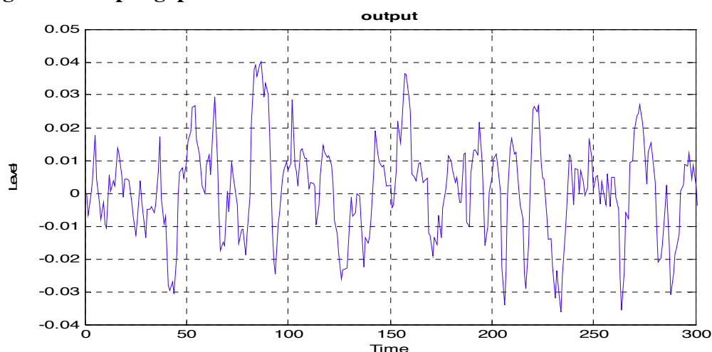
Figure 2: Output gap and inflation in the rational model
