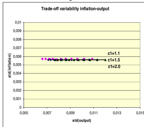
Figure 20: Trade-offs in the simple heuristic model
