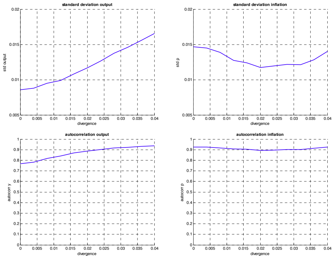
Figure 23: Standard deviation and autocorrelation of output gap and inflation
