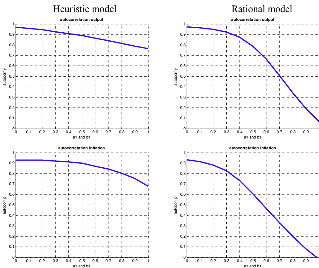
Figure 22: Autocorrelation coefficients of output gap and inflation
