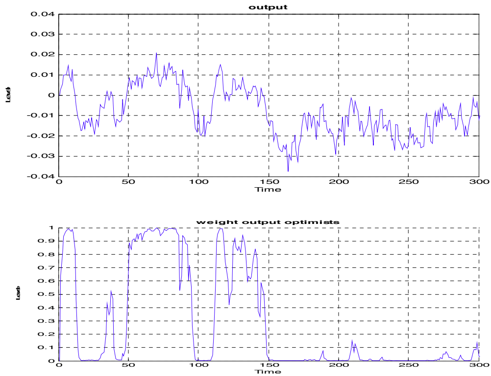
Figure 12: Output in a regime with (imperfectly) credible inflation target
