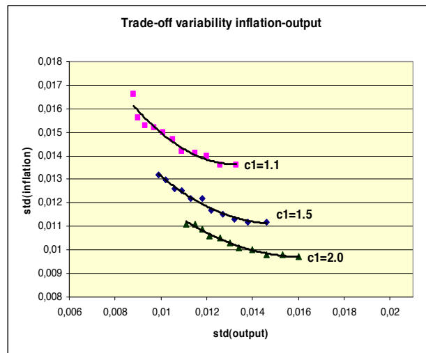
Figure 17: Trade-offs in the extended heuristic model
