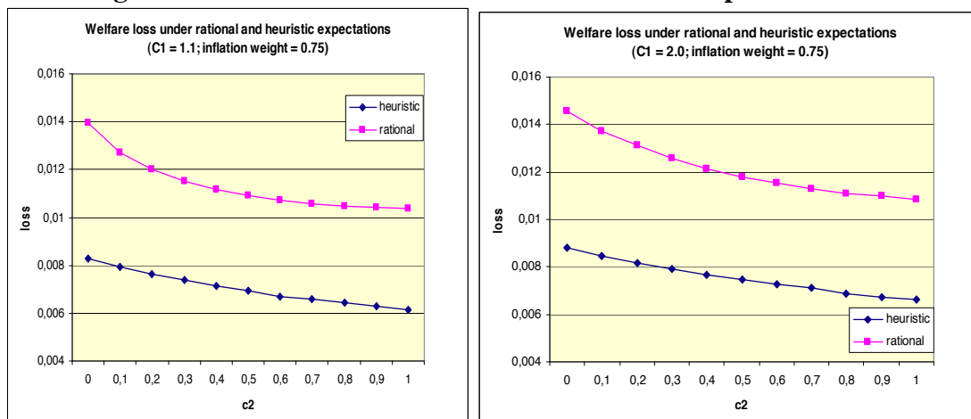
Figure 21: Welfare losses in the rational and the simple heuristic model
