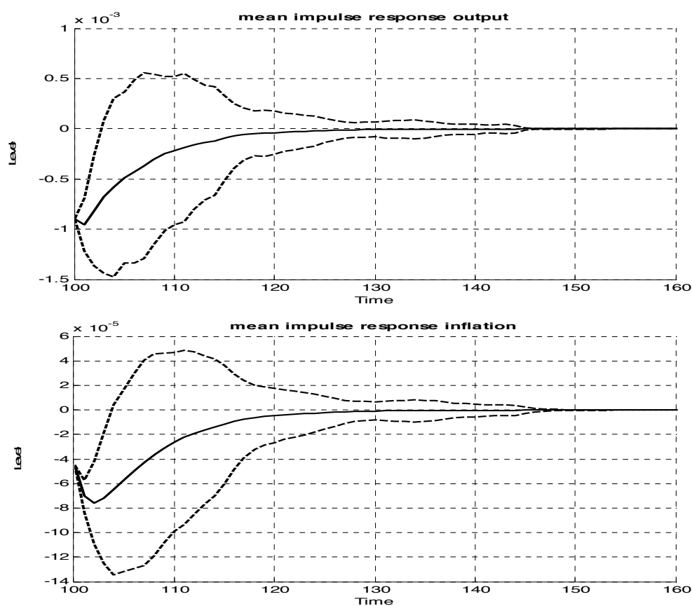
Figure 3: Mean impulse responses to interest rate shock in the heuristic model
