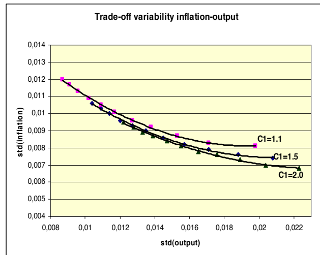
Figure 18: Trade-offs in the rational model
