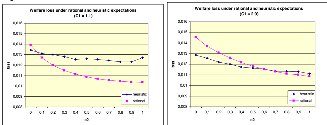
Figure 19: Welfare losses in the rational and the extended heuristic models
