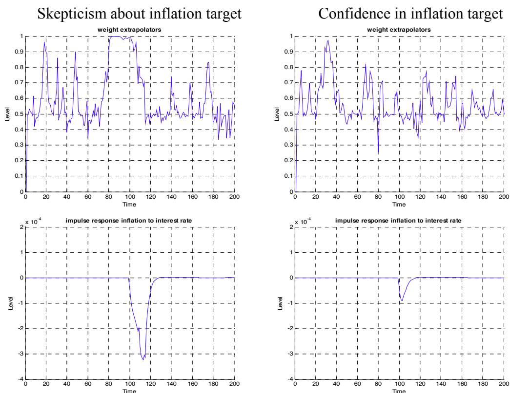
Figure 9: Impulse responses of inflation to interest rate shock (increase)
